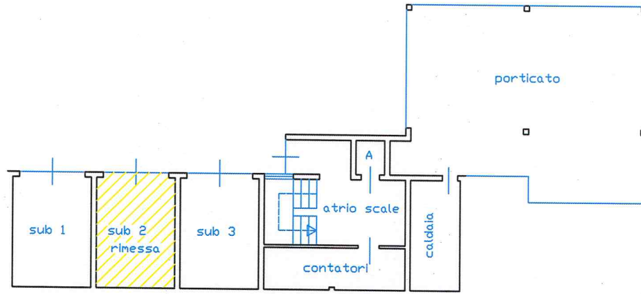
PIANO TERRA
